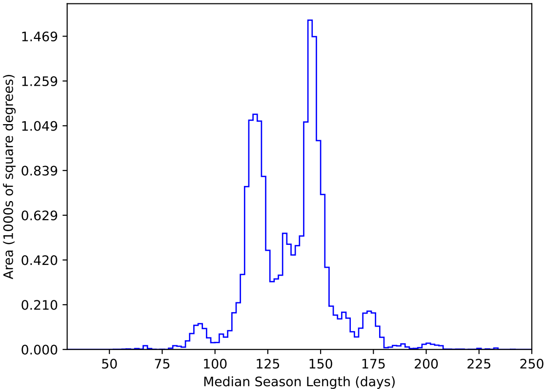
too_elab_heavy_r64_d3_gz_v3.4_10yrs WFD y band: Median Season Length
