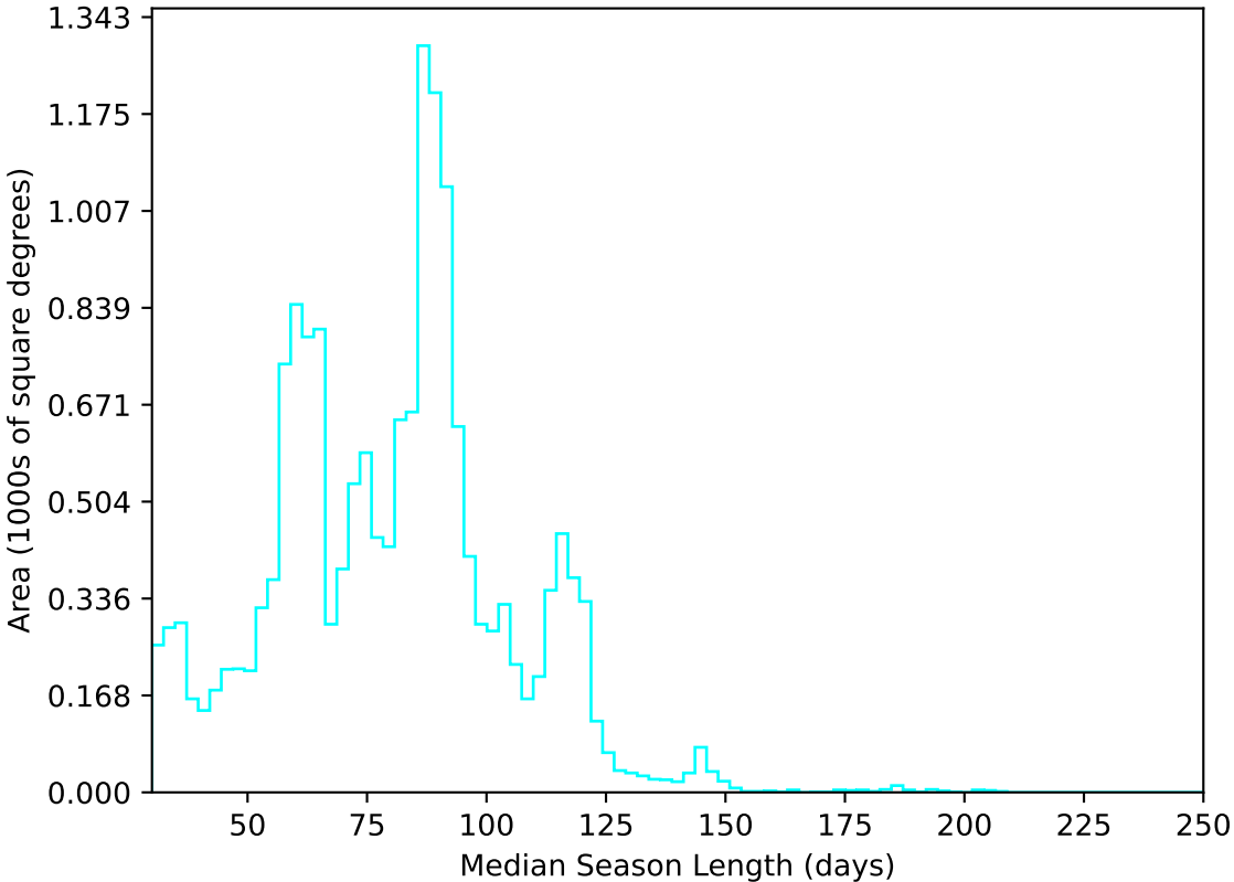
too_elab_heavy_r64_d3_gz_v3.4_10yrs WFD u band: Median Season Length
