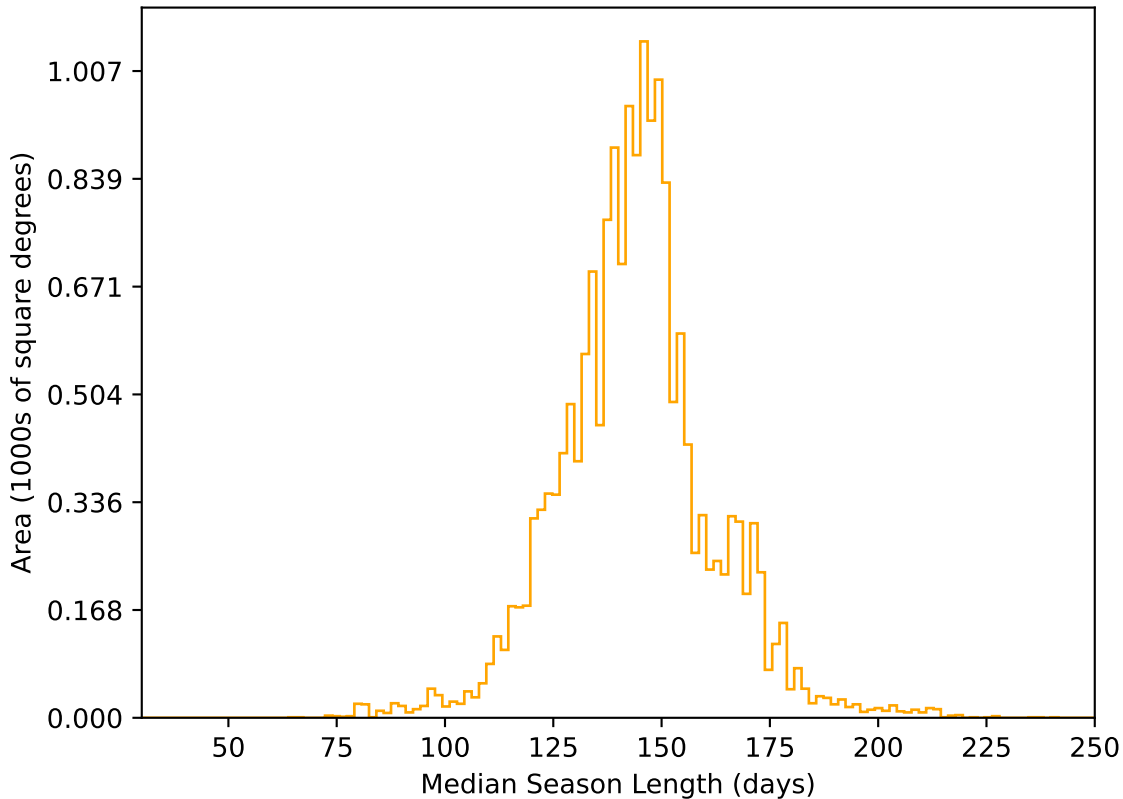
too_elab_heavy_r64_d3_gz_v3.4_10yrs WFD r band: Median Season Length
