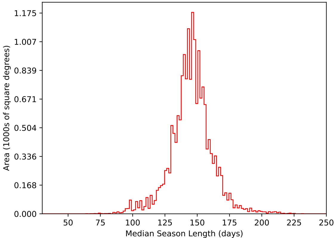
too_elab_heavy_r64_d3_gz_v3.4_10yrs WFD i band: Median Season Length
