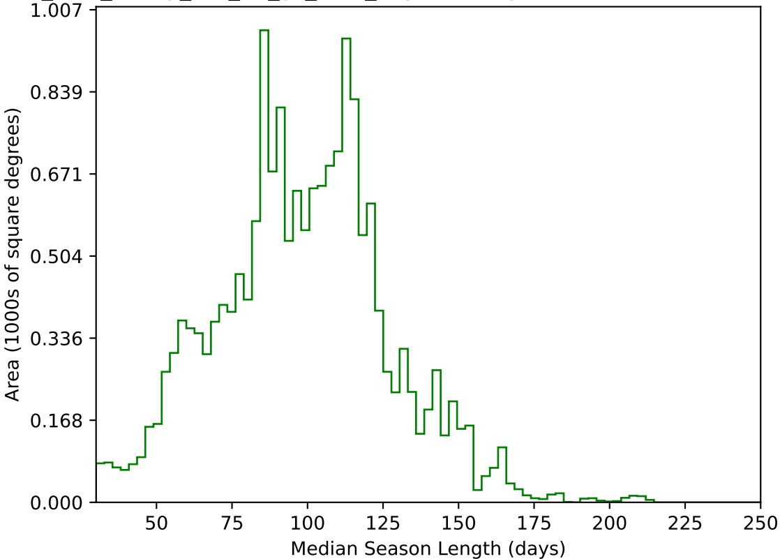
too_elab_heavy_r64_d3_gz_v3.4_10yrs WFD g band: Median Season Length
