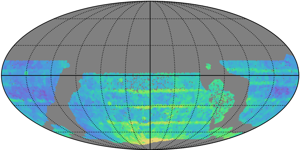
too_elab_heavy_r64_d3_gz_v3.4_10yrs WFD all bands: Median Season Length
