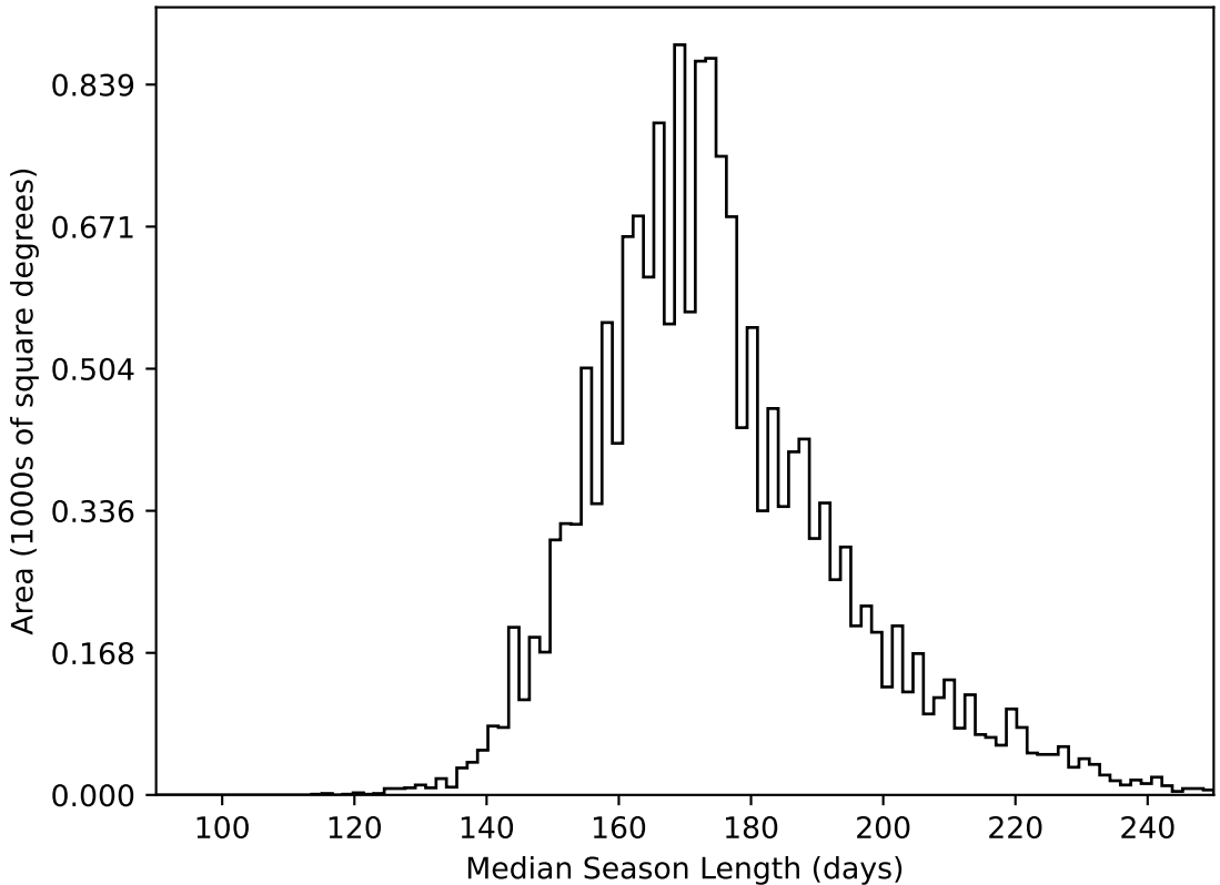
too_elab_heavy_r64_d3_gz_v3.4_10yrs WFD all bands: Median Season Length
