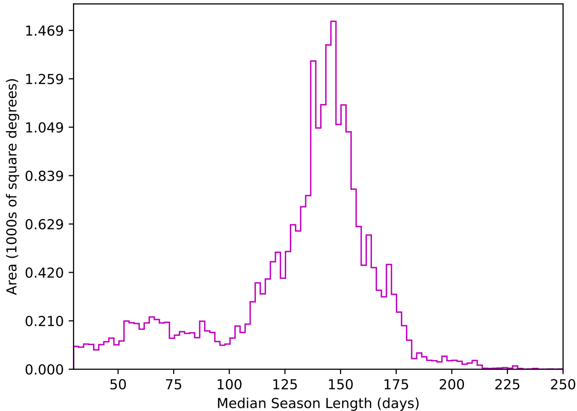
too_elab_heavy_r64_d3_gz_v3.4_10yrs All sky z band: Median Season Length
