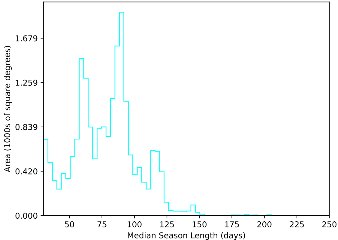
too_elab_heavy_r64_d3_gz_v3.4_10yrs All sky u band: Median Season Length
