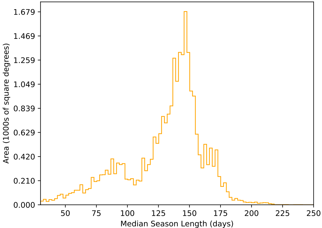
too_elab_heavy_r64_d3_gz_v3.4_10yrs All sky r band: Median Season Length
