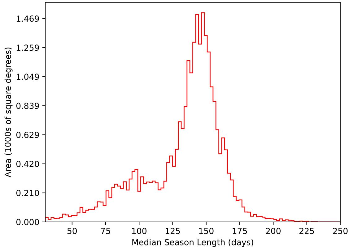
too_elab_heavy_r64_d3_gz_v3.4_10yrs All sky i band: Median Season Length
