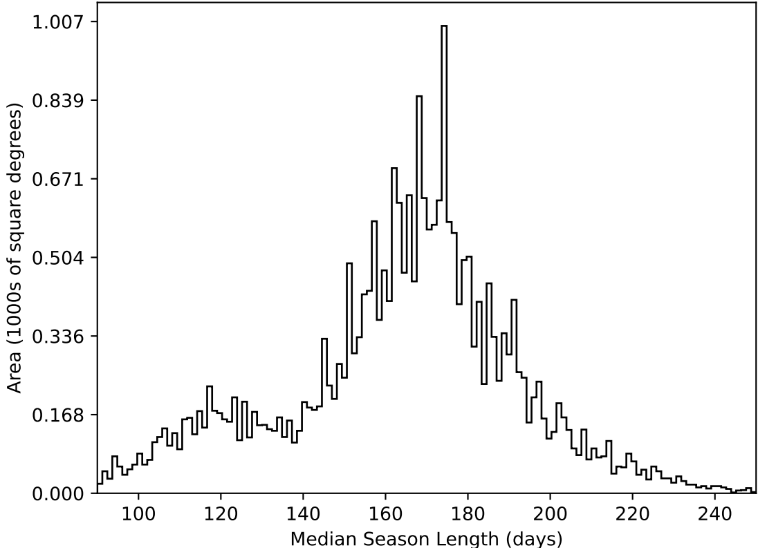
too_elab_heavy_r64_d3_gz_v3.4_10yrs All sky all bands: Median Season Length
