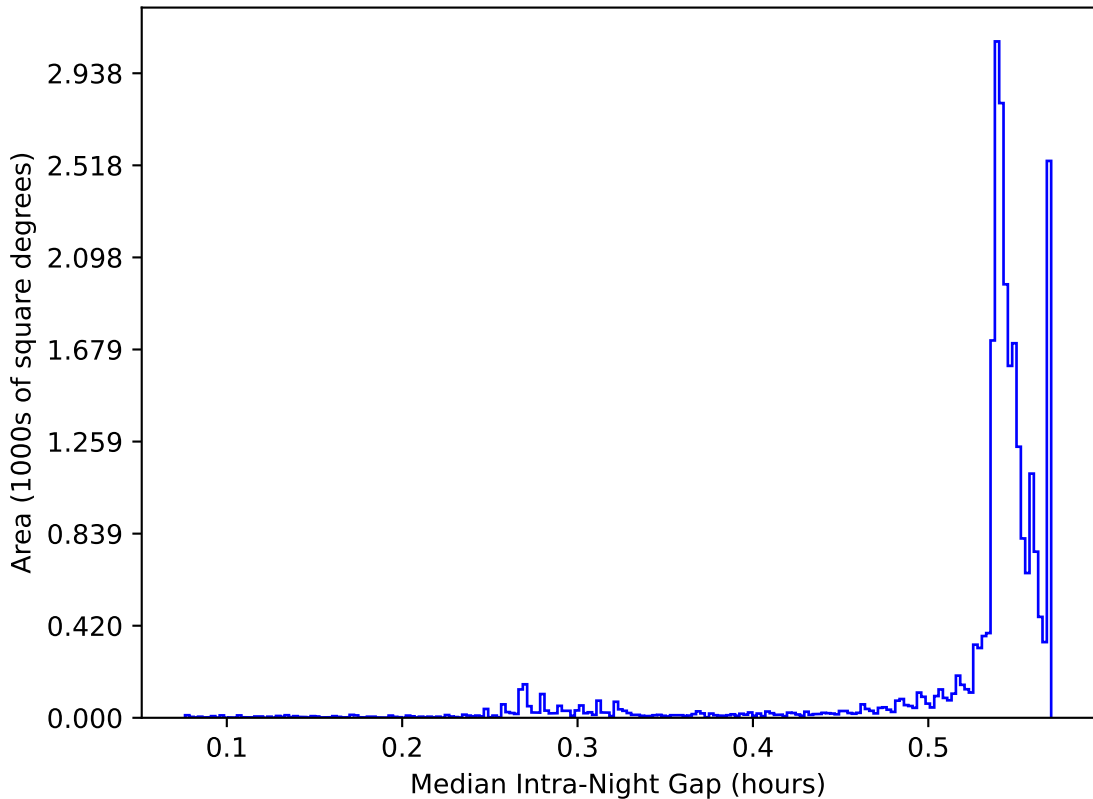
too_elab_heavy_r64_d3_gz_v3.4_10yrs All sky: Median Intra-Night Gap
