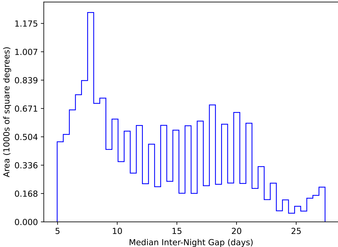
too_elab_heavy_r64_d3_gz_v3.4_10yrs WFD y band: Median Inter-Night Gap
