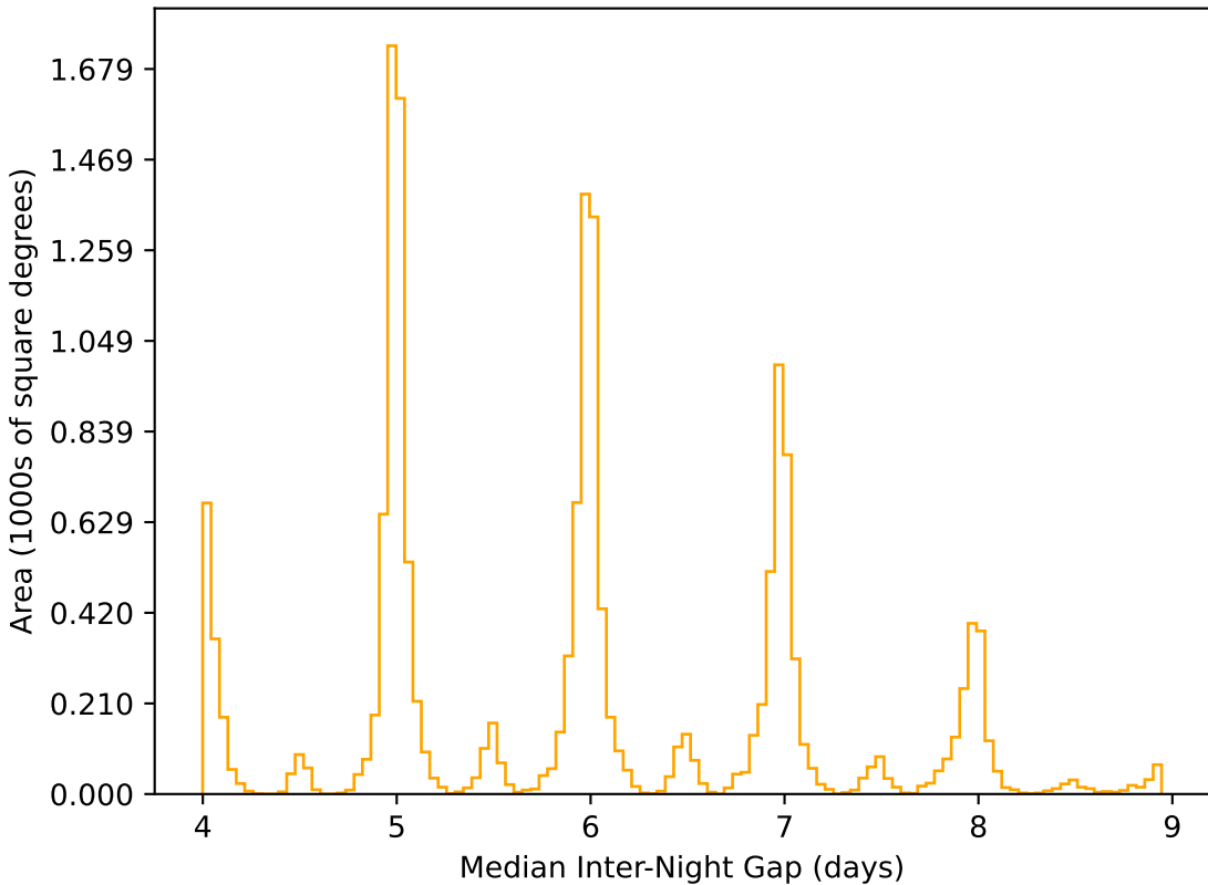
too_elab_heavy_r64_d3_gz_v3.4_10yrs WFD r band: Median Inter-Night Gap
