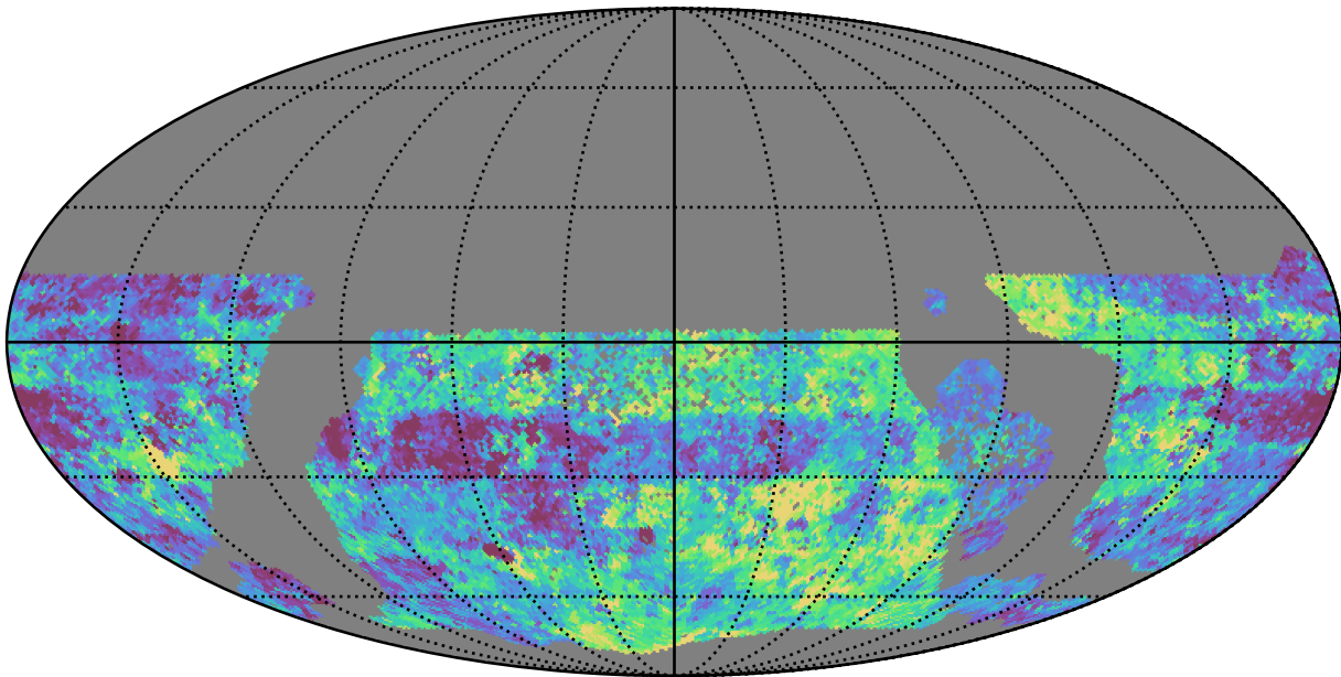
too_elab_heavy_r64_d3_gz_v3.4_10yrs WFD g band: Median Inter-Night Gap
