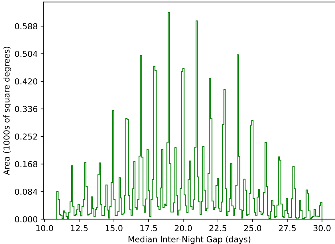
too_elab_heavy_r64_d3_gz_v3.4_10yrs WFD g band: Median Inter-Night Gap
