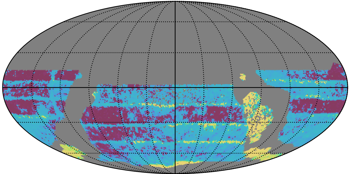
too_elab_heavy_r64_d3_gz_v3.4_10yrs WFD all bands: Median Inter-Night Gap
