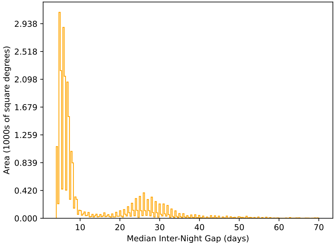
too_elab_heavy_r64_d3_gz_v3.4_10yrs All sky r band: Median Inter-Night Gap
