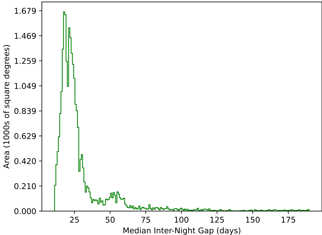
too_elab_heavy_r64_d3_gz_v3.4_10yrs All sky g band: Median Inter-Night Gap
