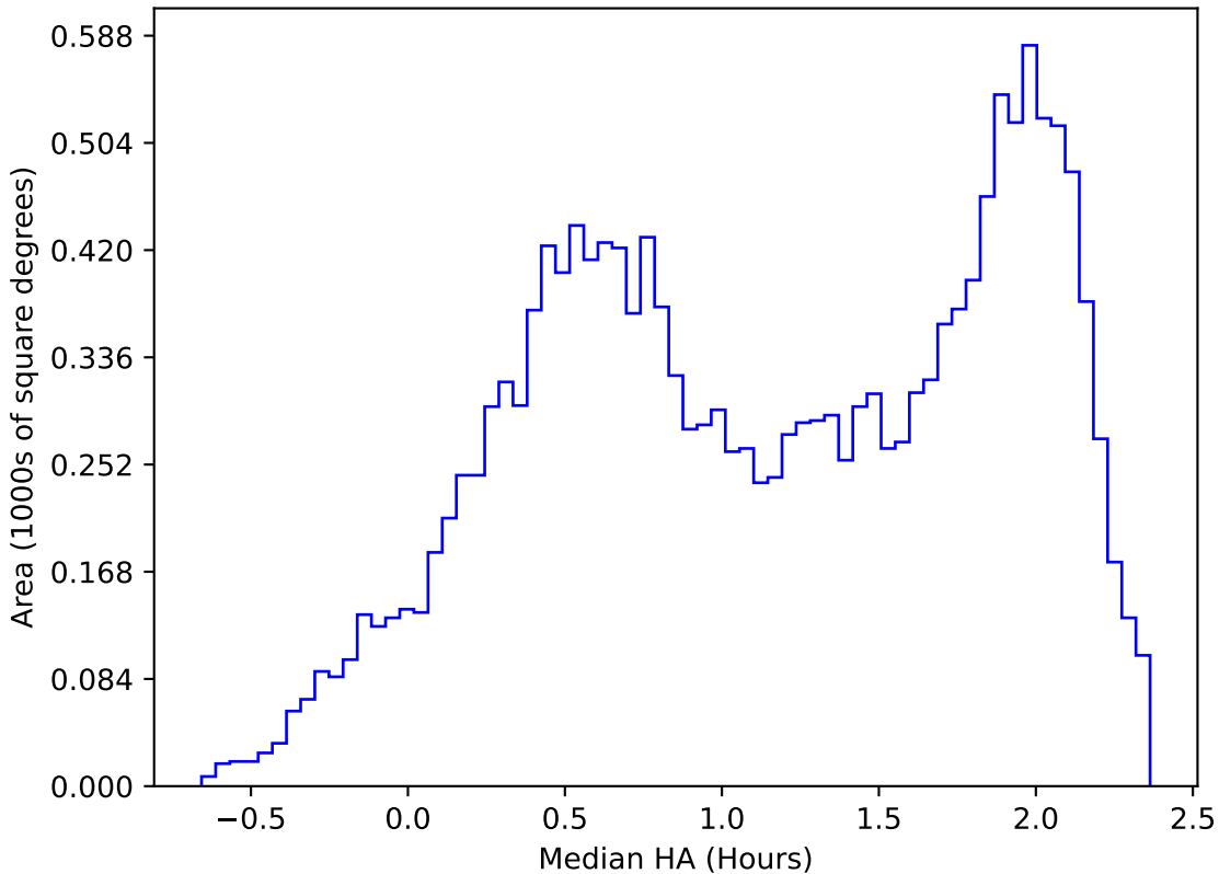
too_elab_heavy_r64_d3_gz_v3.4_10yrs WFD z band: Median HA
