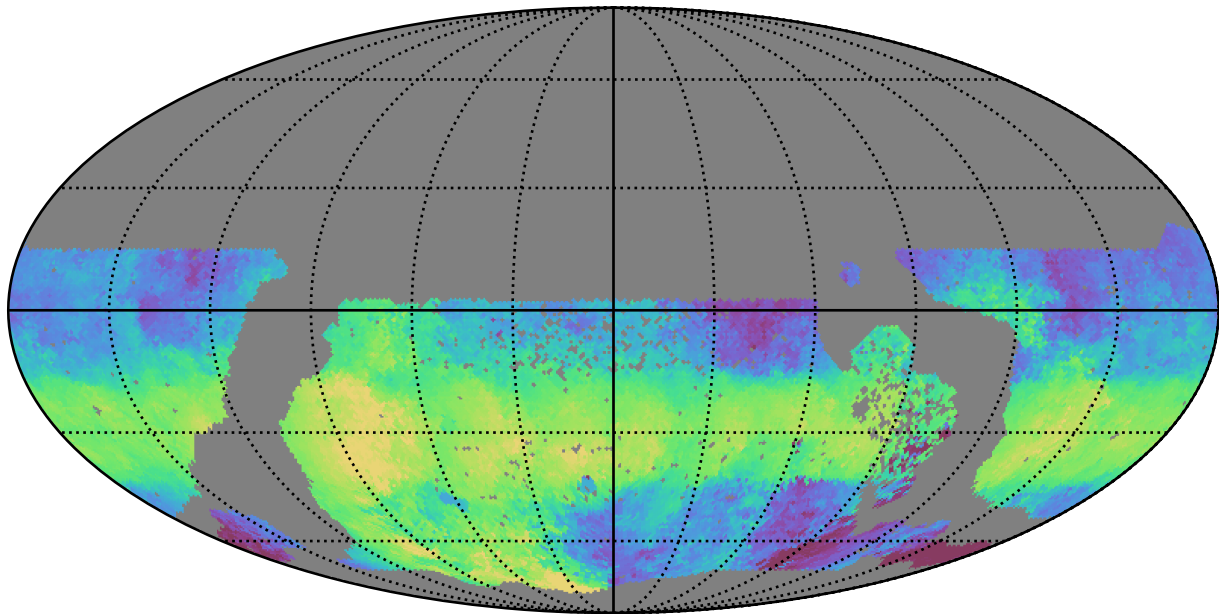
too_elab_heavy_r64_d3_gz_v3.4_10yrs WFD u band: Median HA
