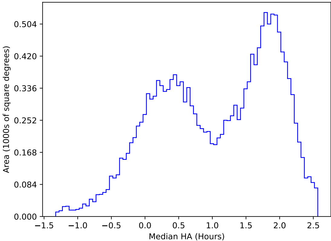
too_elab_heavy_r64_d3_gz_v3.4_10yrs WFD u band: Median HA
