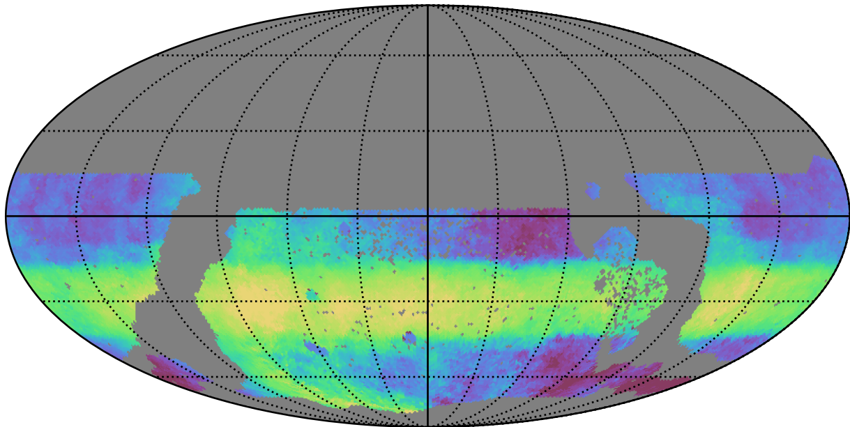
too_elab_heavy_r64_d3_gz_v3.4_10yrs WFD r band: Median HA
