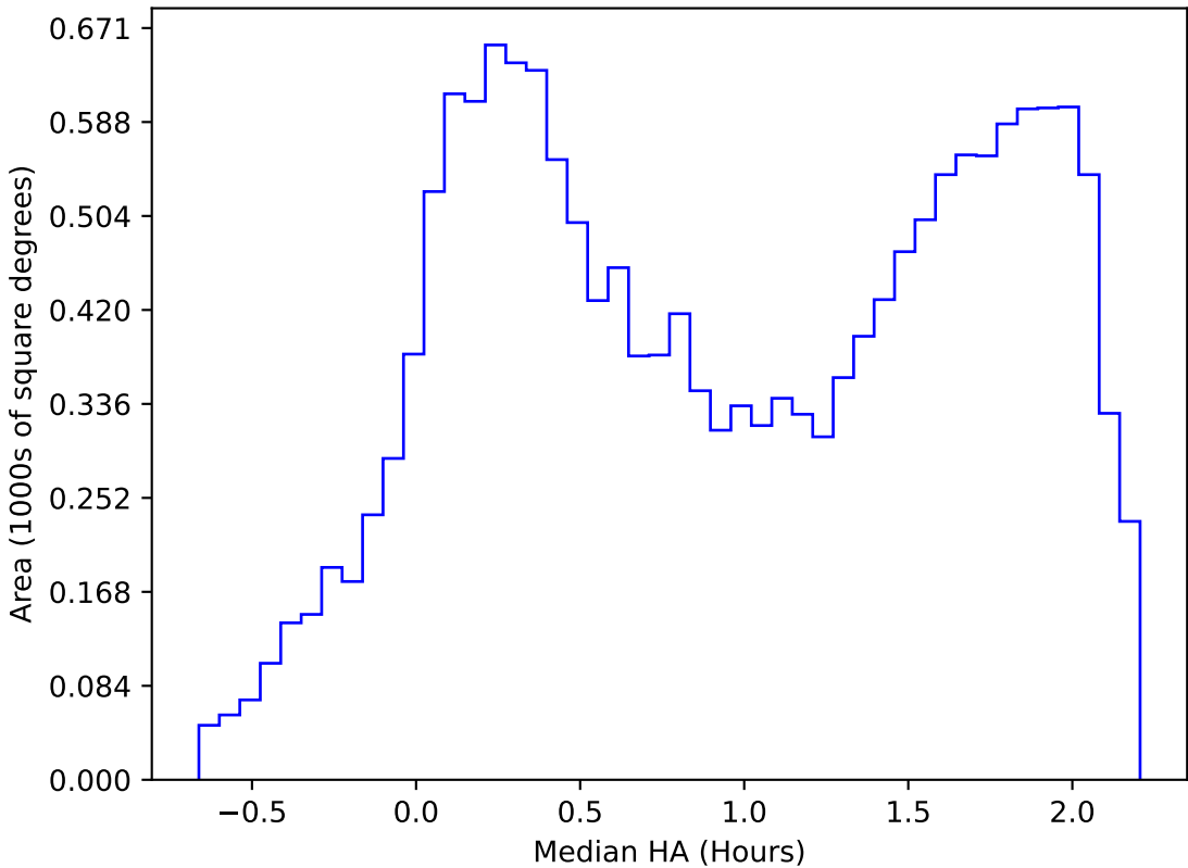
too_elab_heavy_r64_d3_gz_v3.4_10yrs WFD r band: Median HA
