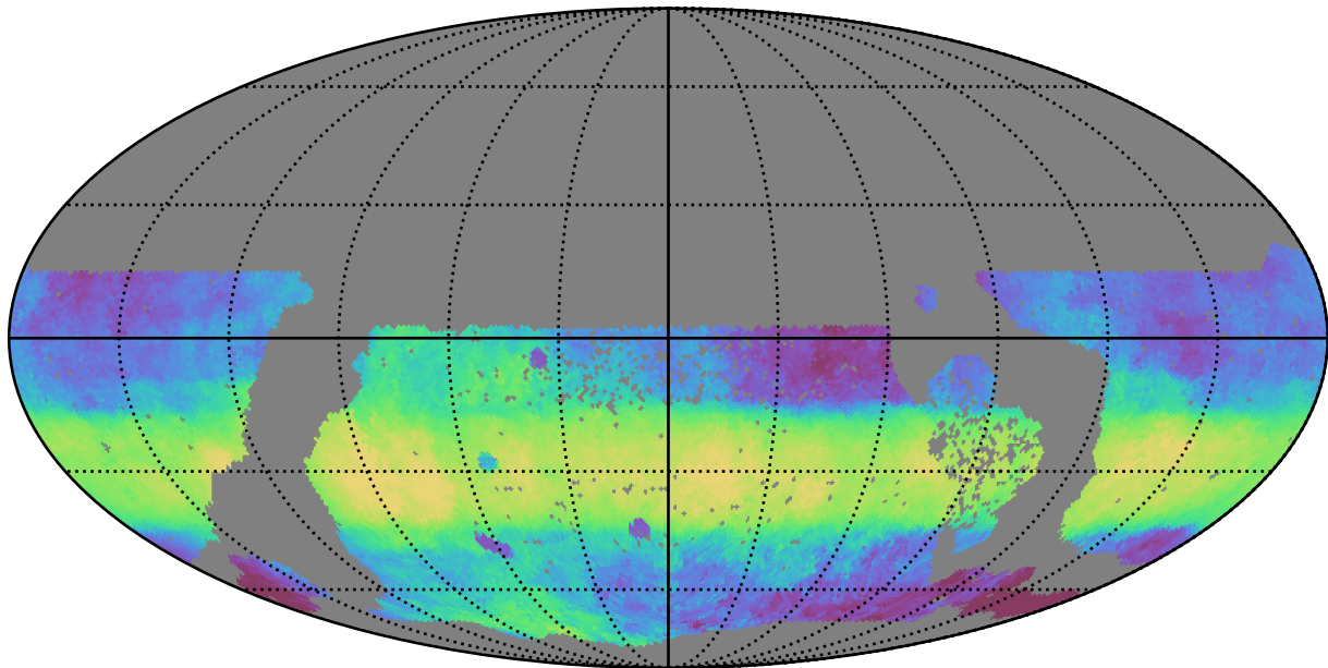
too_elab_heavy_r64_d3_gz_v3.4_10yrs WFD i band: Median HA
