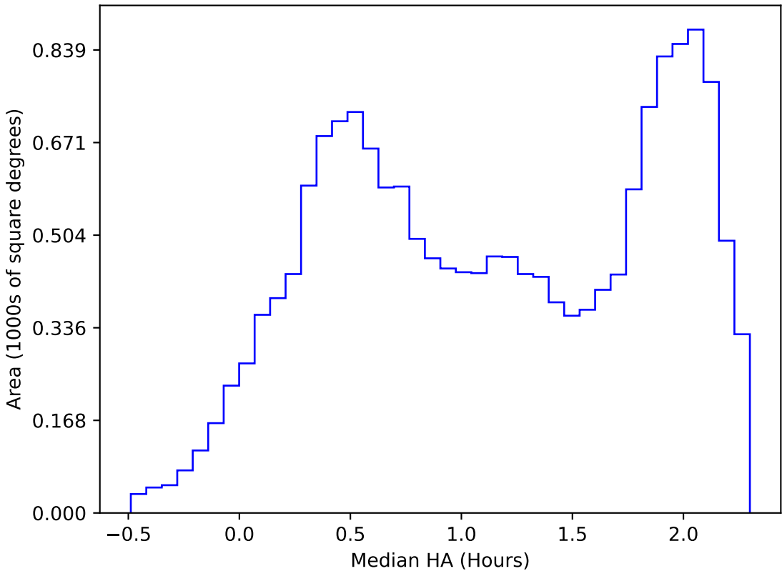
too_elab_heavy_r64_d3_gz_v3.4_10yrs WFD i band: Median HA
