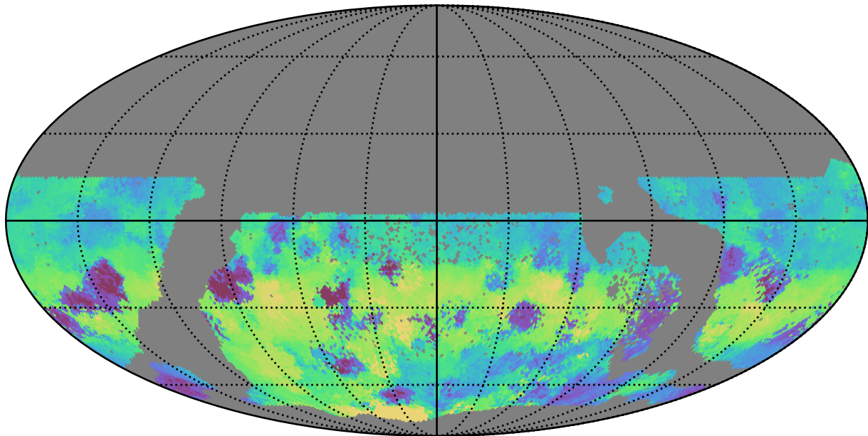
too_elab_heavy_r64_d3_gz_v3.4_10yrs WFD g band: Median HA
