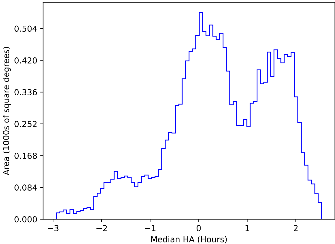
too_elab_heavy_r64_d3_gz_v3.4_10yrs WFD g band: Median HA
