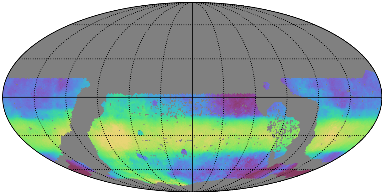
too_elab_heavy_r64_d3_gz_v3.4_10yrs WFD all bands: Median HA
