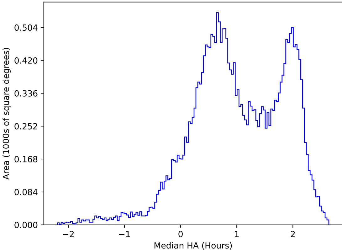
too_elab_heavy_r64_d3_gz_v3.4_10yrs All sky z band: Median HA
