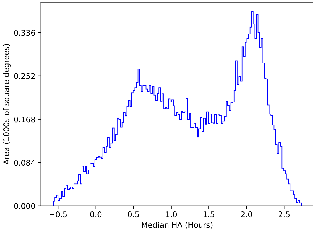
too_elab_heavy_r64_d3_gz_v3.4_10yrs All sky y band: Median HA
