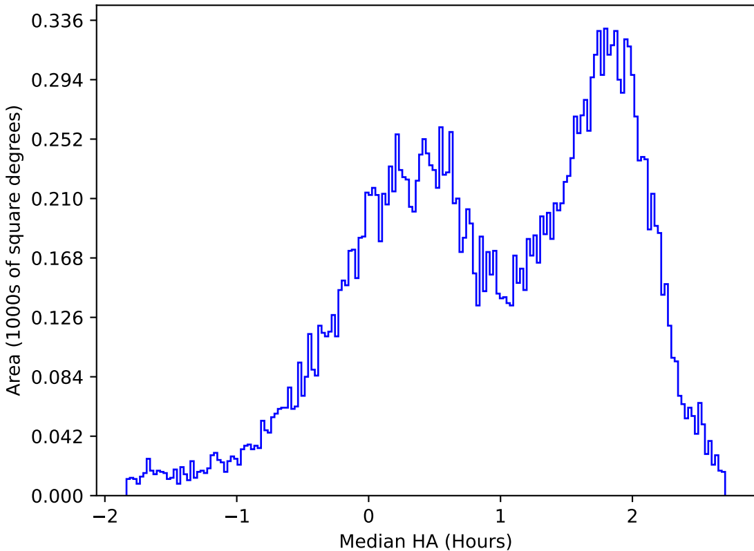
too_elab_heavy_r64_d3_gz_v3.4_10yrs All sky u band: Median HA
