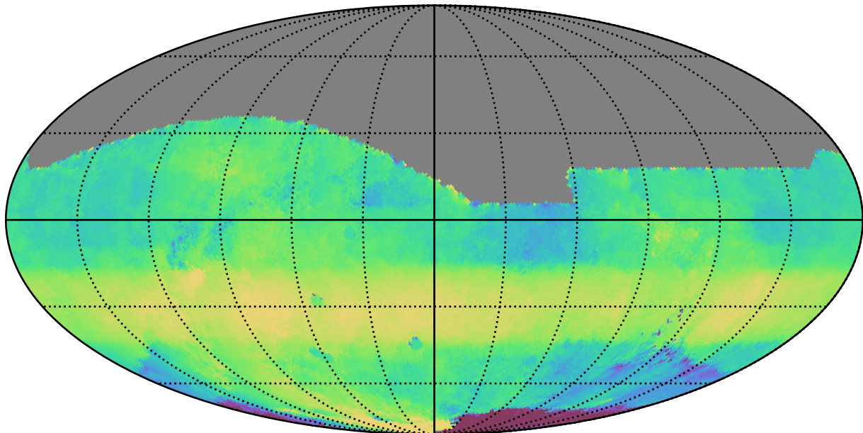
too_elab_heavy_r64_d3_gz_v3.4_10yrs All sky r band: Median HA
