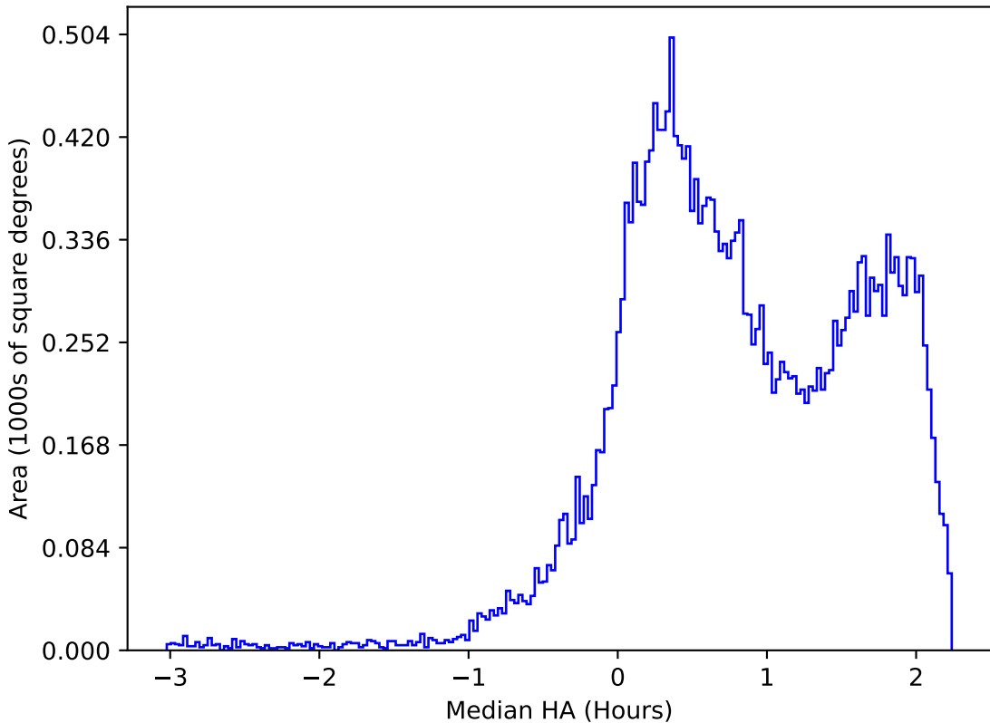
too_elab_heavy_r64_d3_gz_v3.4_10yrs All sky r band: Median HA
