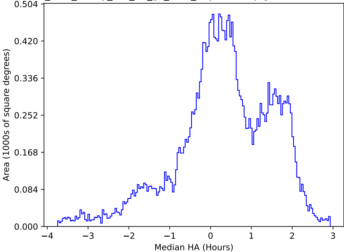
too_elab_heavy_r64_d3_gz_v3.4_10yrs All sky g band: Median HA
