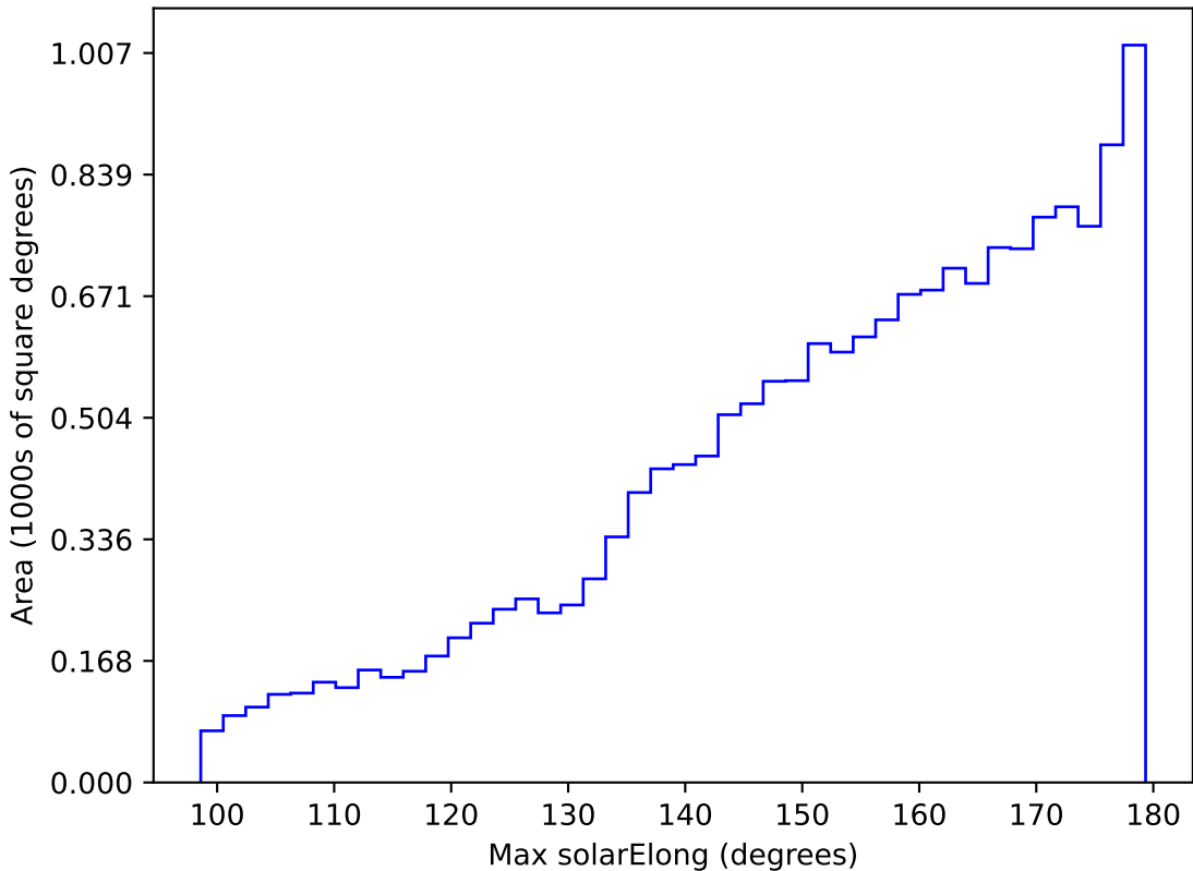
too_elab_heavy_r64_d3_gz_v3.4_10yrs WFD z band: Max solarElong
