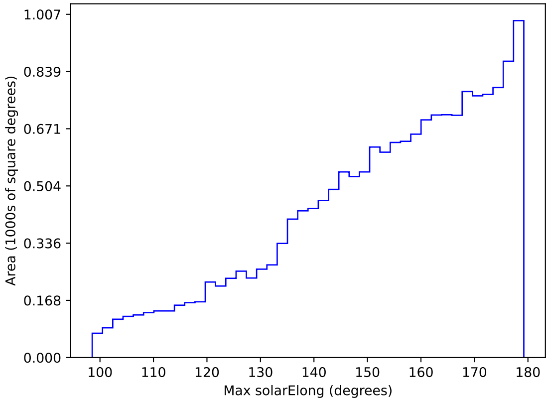
too_elab_heavy_r64_d3_gz_v3.4_10yrs WFD y band: Max solarElong
