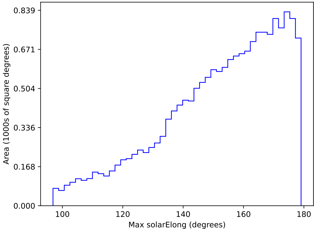
too_elab_heavy_r64_d3_gz_v3.4_10yrs WFD u band: Max solarElong
