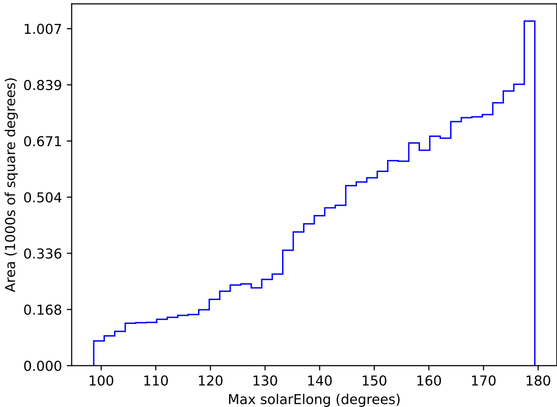
too_elab_heavy_r64_d3_gz_v3.4_10yrs WFD r band: Max solarElong
