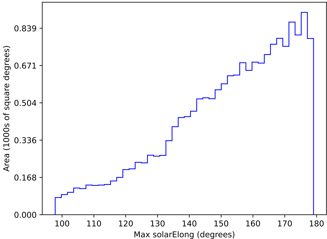
too_elab_heavy_r64_d3_gz_v3.4_10yrs WFD g band: Max solarElong
