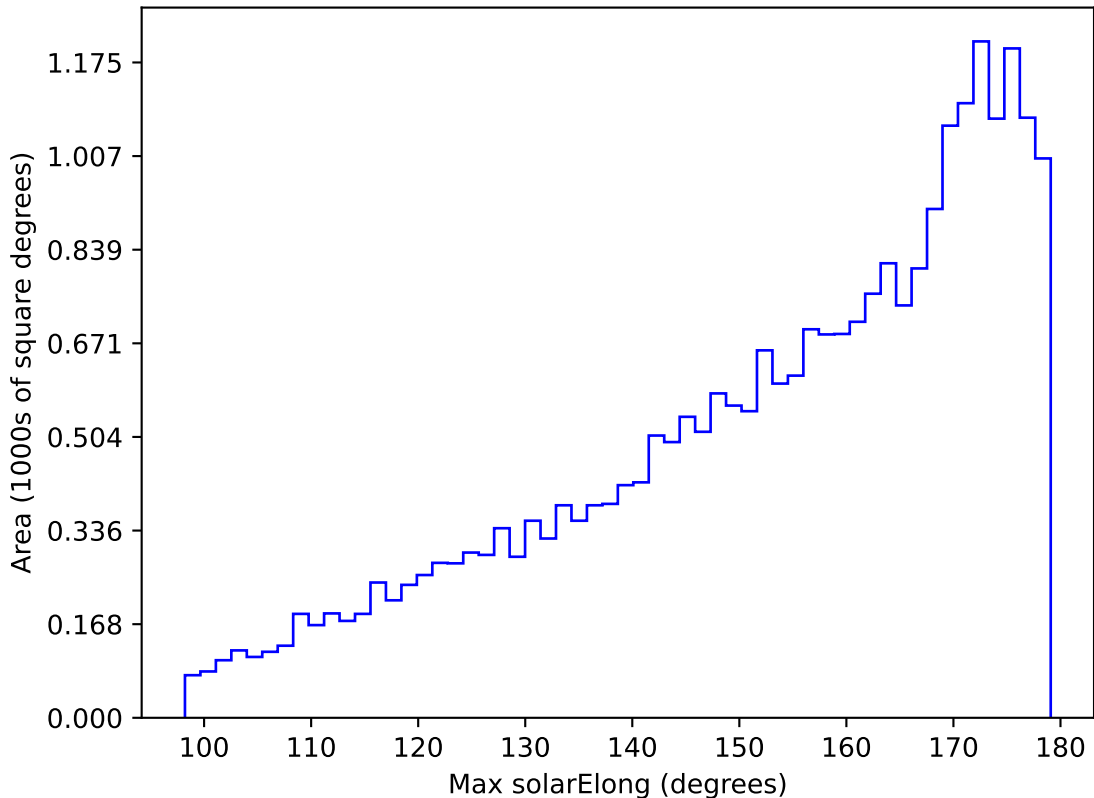
too_elab_heavy_r64_d3_gz_v3.4_10yrs All sky g band: Max solarElong
