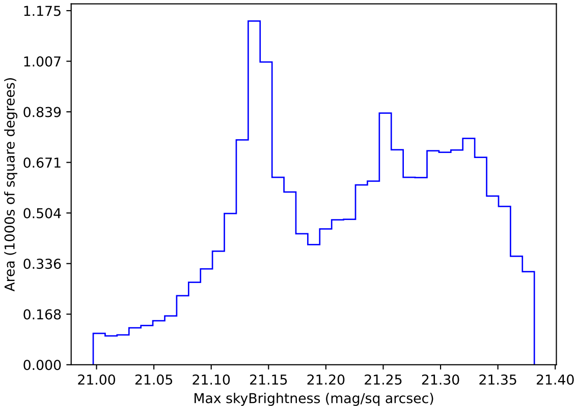
too_elab_heavy_r64_d3_gz_v3.4_10yrs WFD r band: Max skyBrightness
