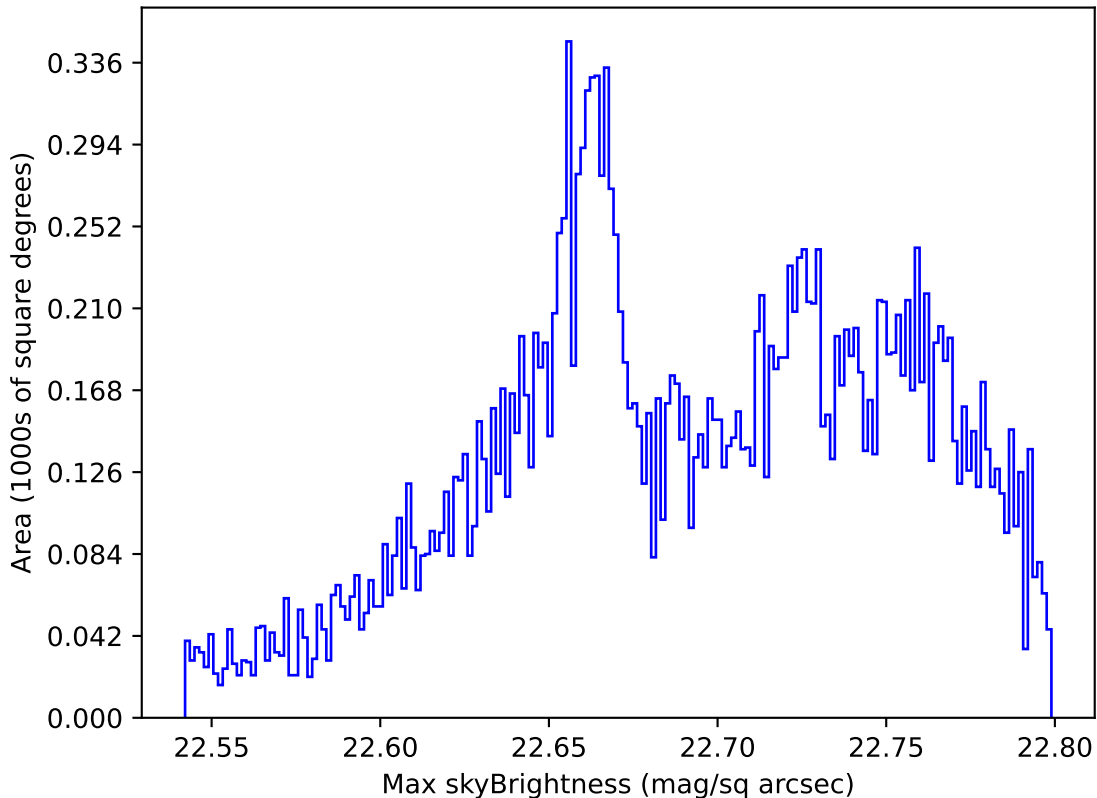
too_elab_heavy_r64_d3_gz_v3.4_10yrs All sky u band: Max skyBrightness
