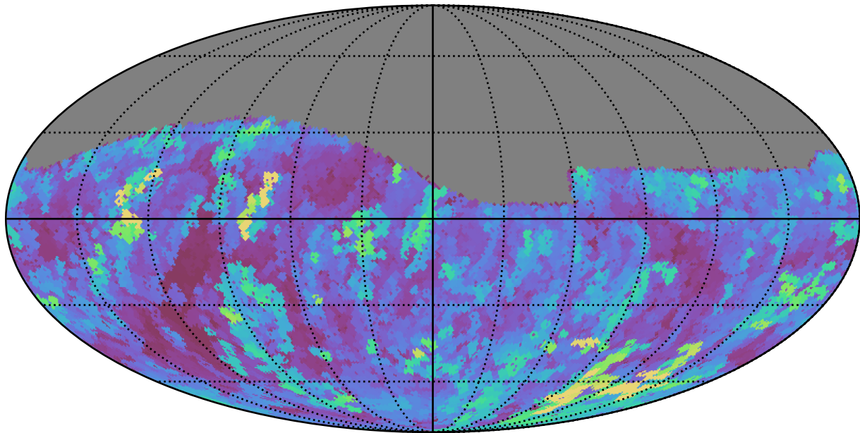
too_elab_heavy_r64_d3_gz_v3.4_10yrs Yr 1 r band: Max seeingEff
