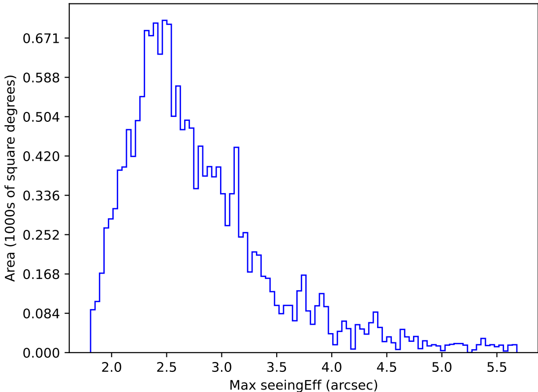
too_elab_heavy_r64_d3_gz_v3.4_10yrs WFD i band: Max seeingEff
