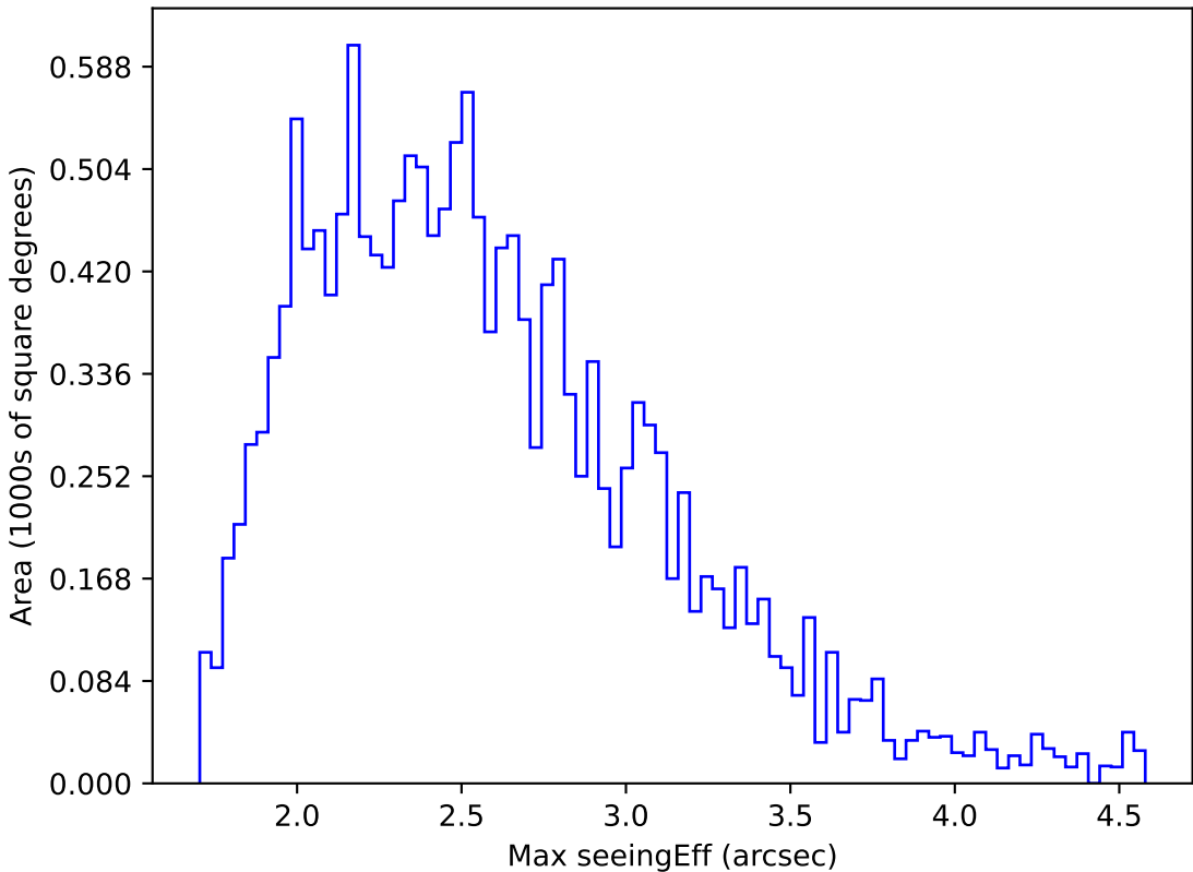
too_elab_heavy_r64_d3_gz_v3.4_10yrs WFD g band: Max seeingEff
