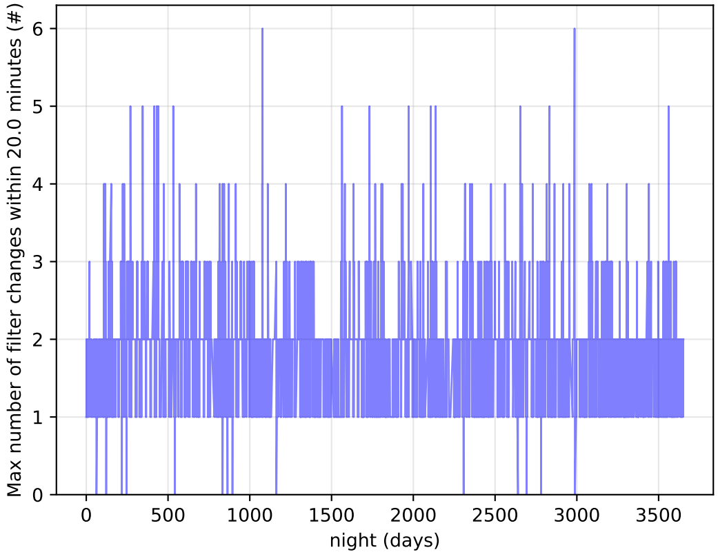
too_elab_heavy_r64_d3_gz_v3.4_10yrs Per Night: Max number of filter changes within 20.0 minutes
