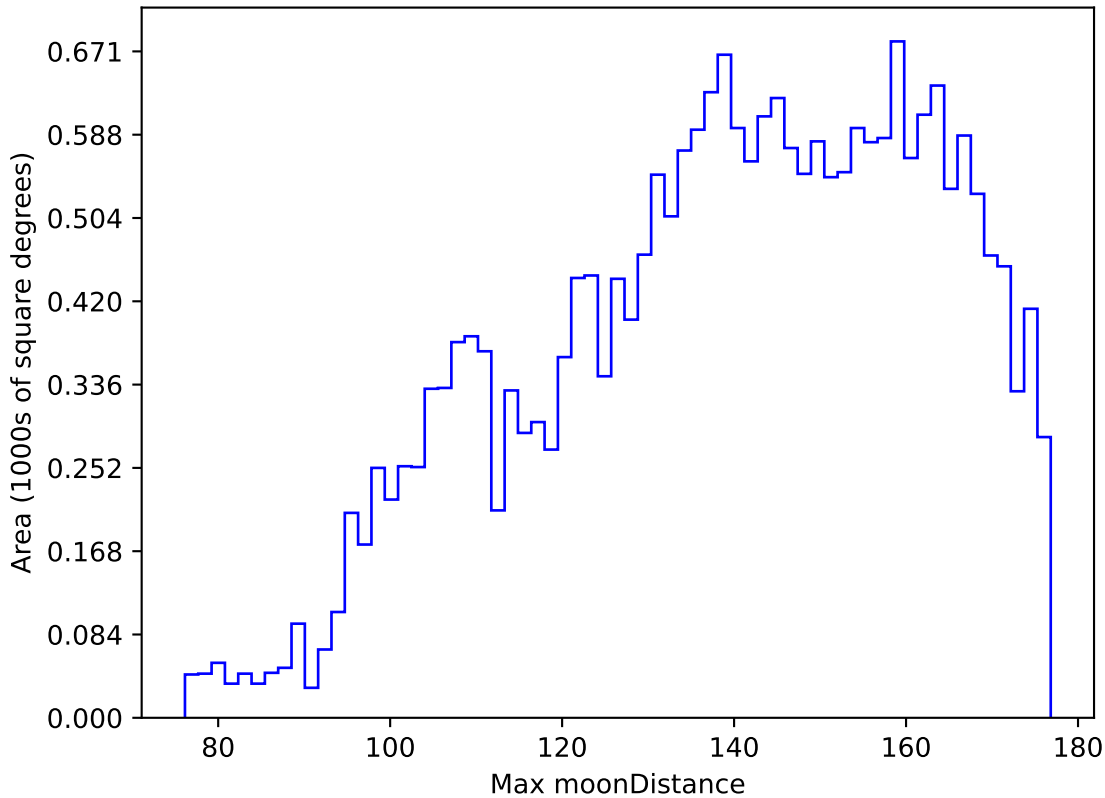
too_elab_heavy_r64_d3_gz_v3.4_10yrs All sky y band: Max moonDistance
