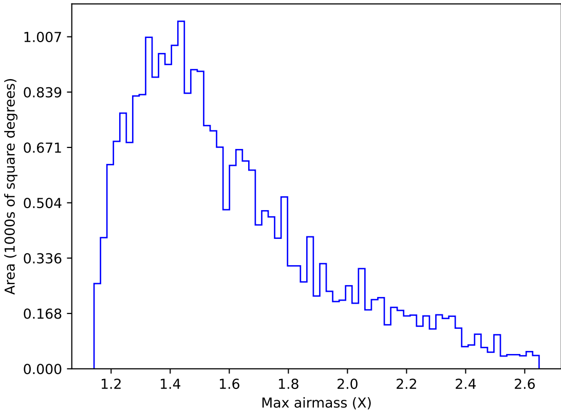
too_elab_heavy_r64_d3_gz_v3.4_10yrs Yr 1 z band: Max airmass
